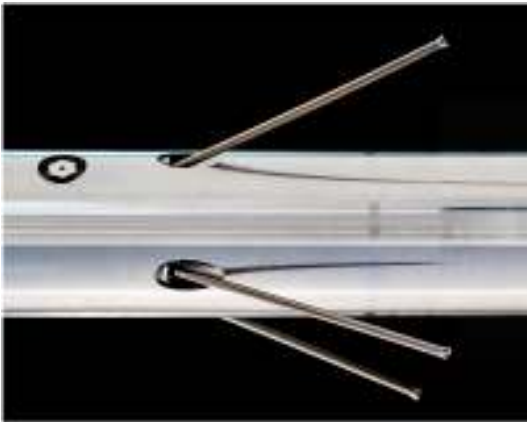
Fishbones Sub with Production Valve and Needles
